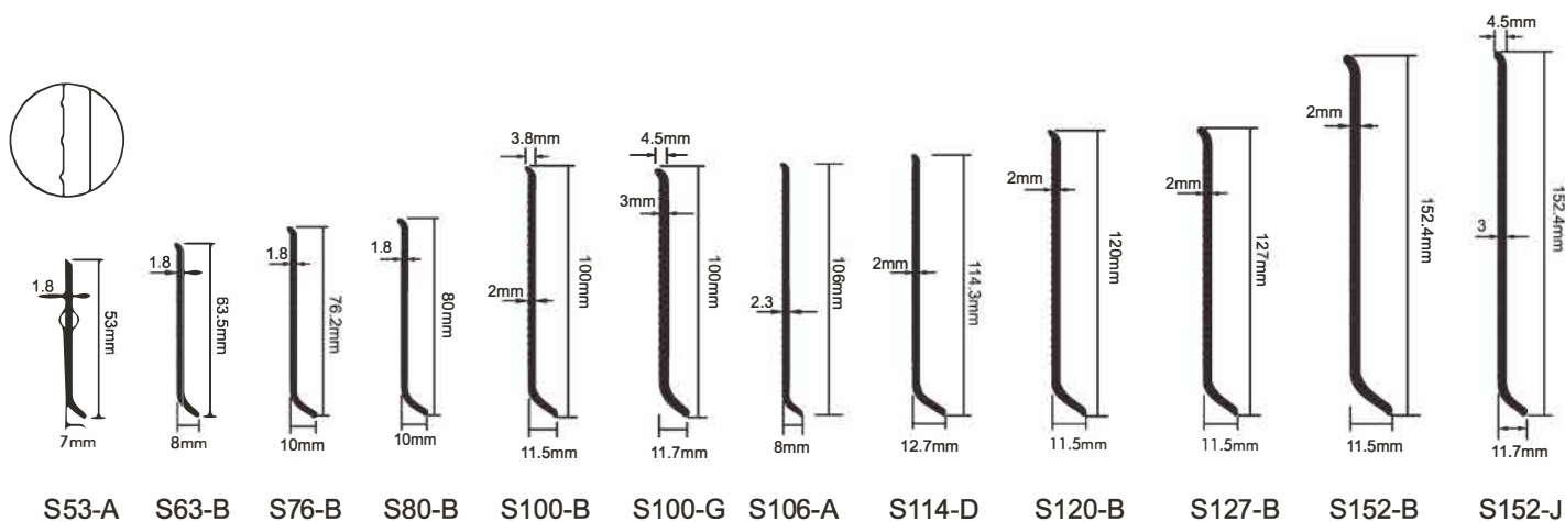
VWB-001 series-Convex back design
