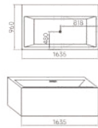
Size:1635×960×610mm
