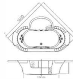
Size:1650*1600*480mm
