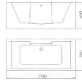
Size:1700 ×780 ×650mm
