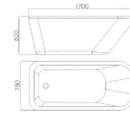
Size:1700×780×600mm
