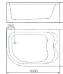
Size:1800 ×1240 ×680mm
