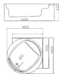
Size:1650*1650*620mm
