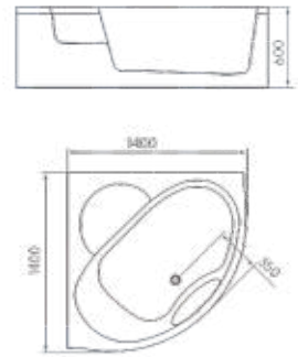
Size:1400 ×1400 ×600mm
