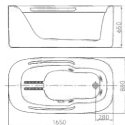
Size:1650*880*650mm
