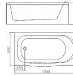
Size:1700 ×880 ×585mm
