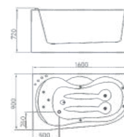
Size:1600*900*720mm
