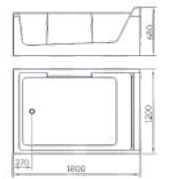
Size:1800 ×1200 ×680mm
