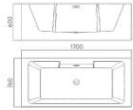
Size:1700×760×600mm
